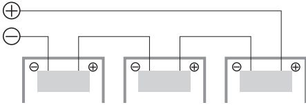
Series Wiring (Voltage Additive)
