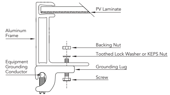
Figure 8: Grounding lug detail
