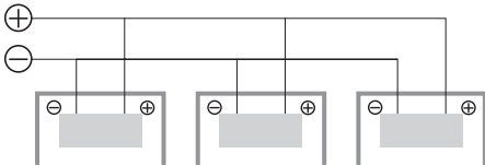
Parallel Wiring (Current Additive)
