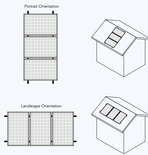
Figure 10: Landscape and portrait mounting
