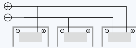
Parallel Wiring (Current Additive)
