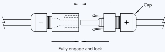
Figure 5: Series interconnection of a male (-) and female (+) connector
