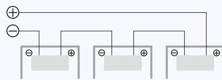
Series Wiring (Voltage Additive)
